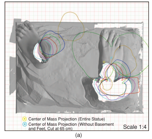
Fig. 2 Spatial location of David's barycenter (a) with and without basement and feet; (b) zoomed images.
