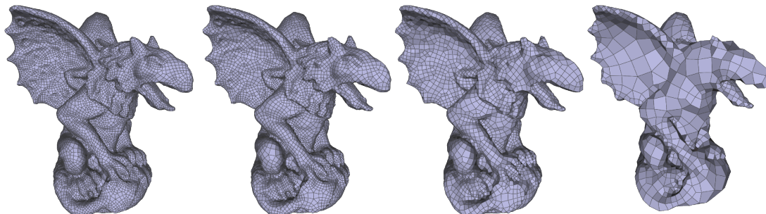
Figure 4: The gargoyle datasets simplified at 18k, 12k and 6k faces. The adaptivity of the mesh increases during the simplification.
