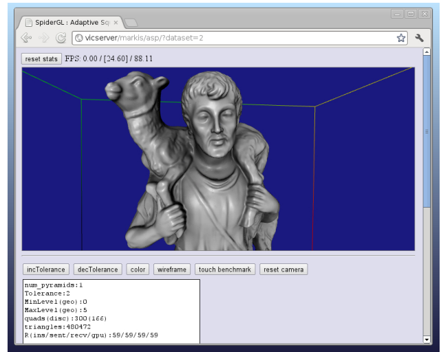
Figure 8: WebGL implementation running in Chrome. 3D content can be delivered in a HTML5 canvas. Models are incrementally loaded during rendering.
