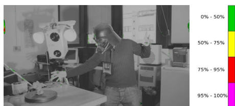
Figure 4: An example of HDR-VDP comparison between frames of an HD video generated using the CPU version of the algorithm and our novel method. The HDR-VDP error is less than 1%.
