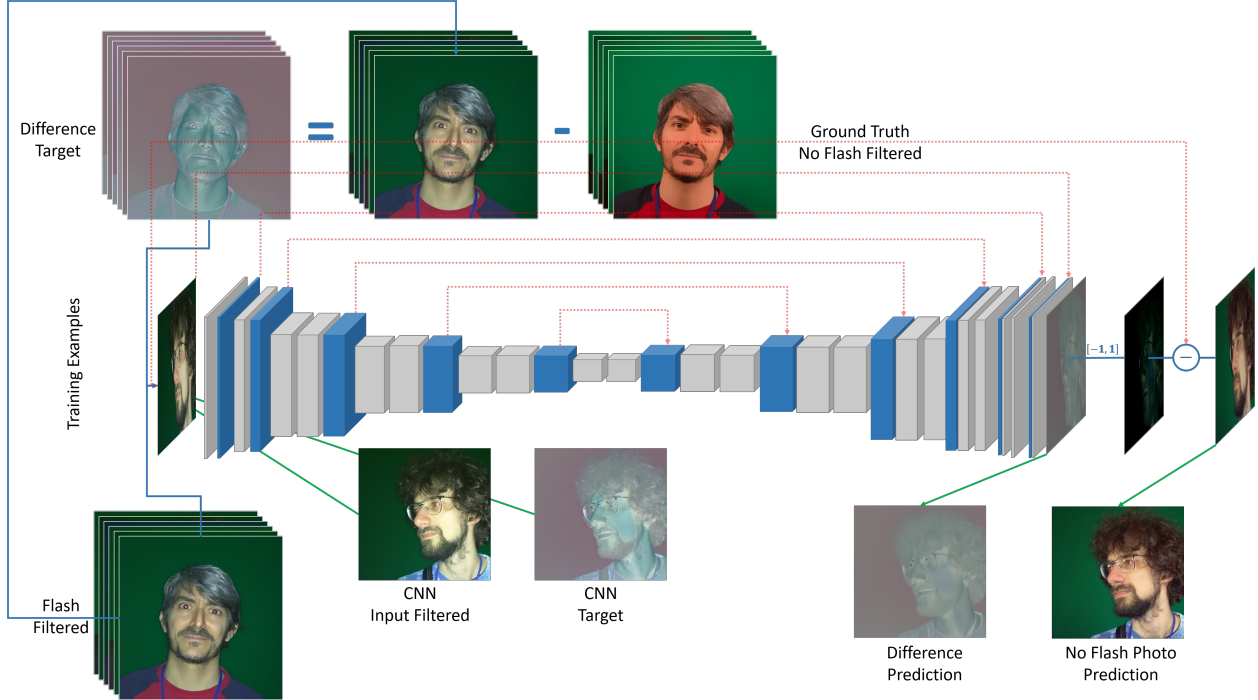
Figure 2: Our neural network architecture for transforming a flash image into a non-flash image. The first 13 blocks represent the VGG-16’s convolutional layers, which perform the image encoding. The second part reconstructs the output image and has several convolutional and deconvolutional layers. From the blue blocks of the VGG-16, the shortcut connections start, which are linked with their counterparts in the decoder. The CNN input is an image taken with the smartphone flash, and the ground truth is an image taken using simulated ambient light, on both of which the bilateral filter is applied. The target image is the difference between the input and ground truth image, normalized in a range between 0 and 1. The network prediction is the searched difference, which is denormalized in the range [-1, 1] and then subtracted from the non-filtered input. The final output prediction is an image without flash highlights.
