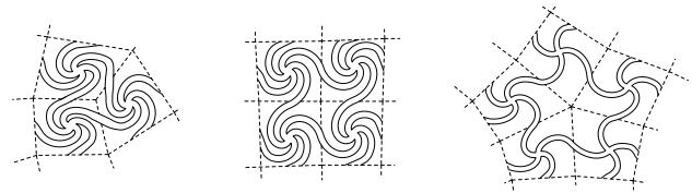
Figure 2: Connections between the spirals in the case of 3 quads (singularity), 4 quads (regular case), 5 quads (singularity).
